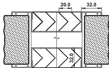
ALL DIMENSION IN mm. (FIGURE 22)
