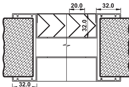
ALL DIMENSION IN mm. (FIGURE 21)
